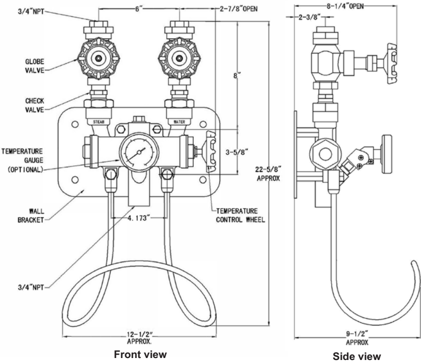
Duramix 8000 Technical Drawings
